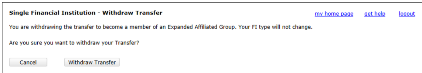
Figure 71 – Withdraw transfer
