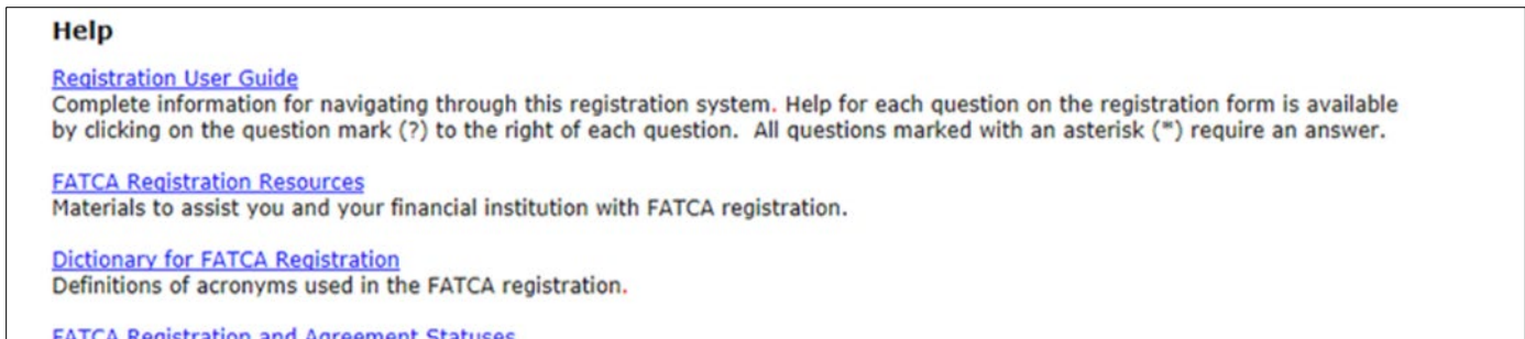
Figure 96 – Help page
