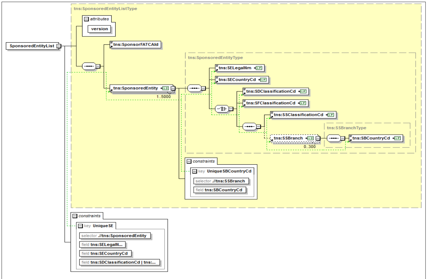
Figure 97 – Sponsored entity list schema diagram
